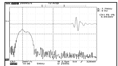
10 MHz. 16 vpp. ZERO dB amplification
