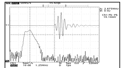
3 MHz. 16 vpp. ZERO dB amplification
